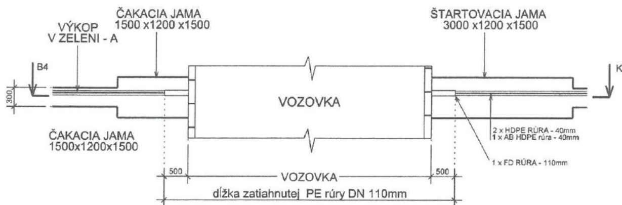
REZ K-K
